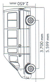
Citroën Jumper Minibus Longo
